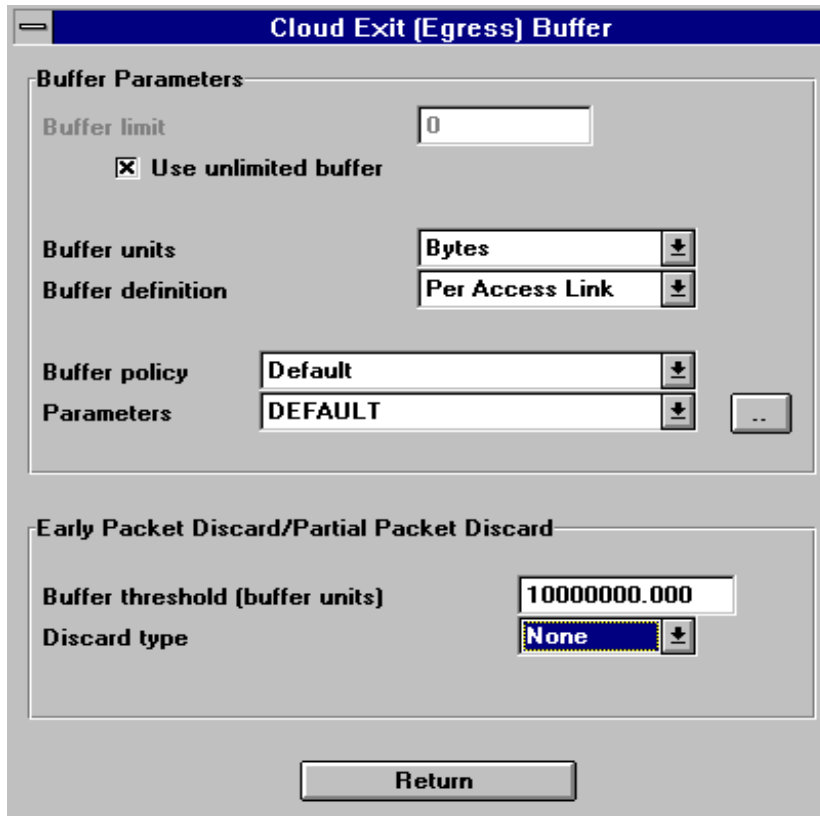
Figure 8.5a Cloud Exit (Egress) Buffer Parameters
